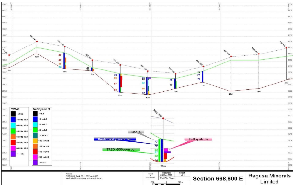
Figure 3. Section 668,600 East
