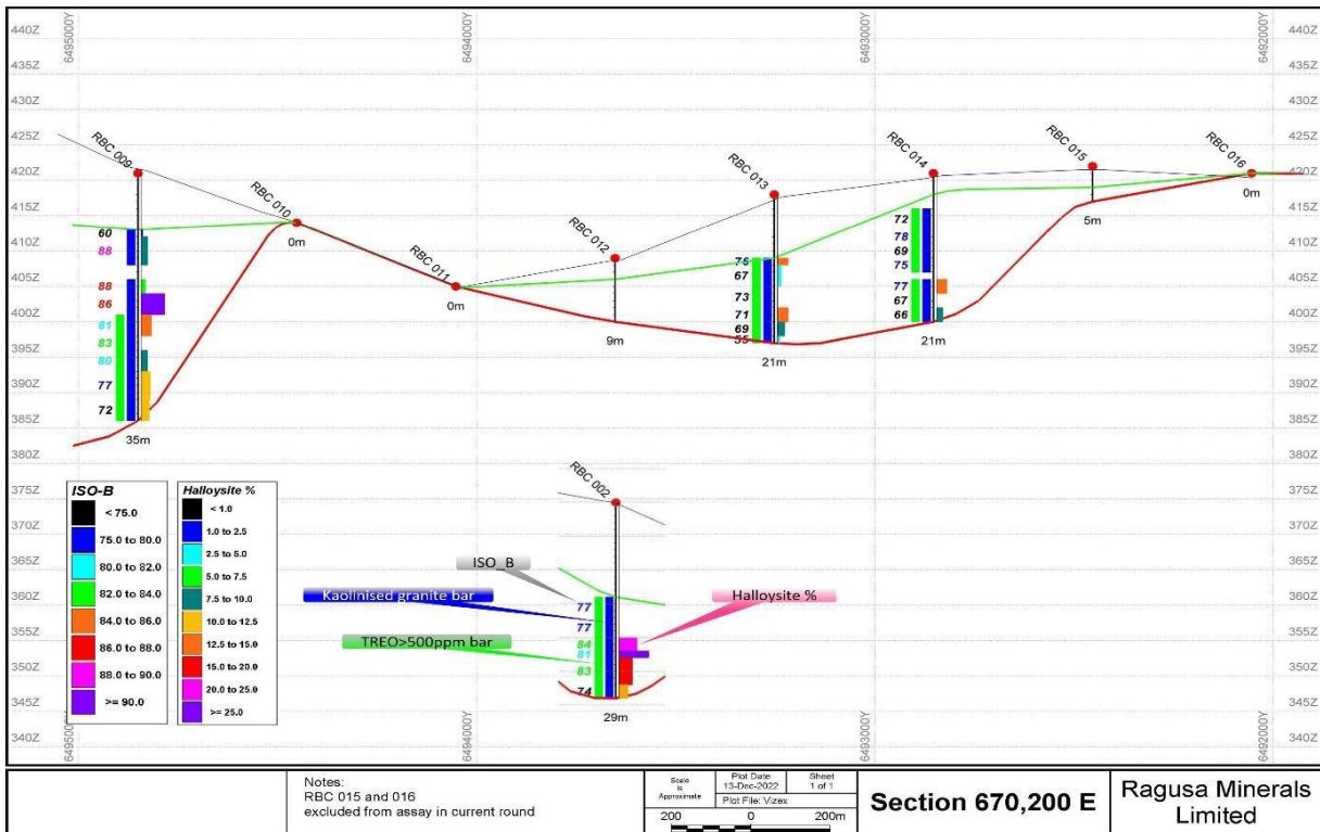
Figure 7. Section 670,200 East
