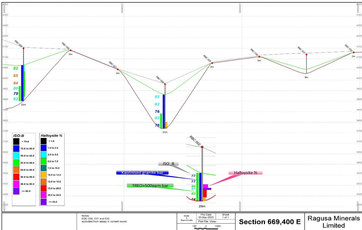
Figure 5. Section 669,400 East
