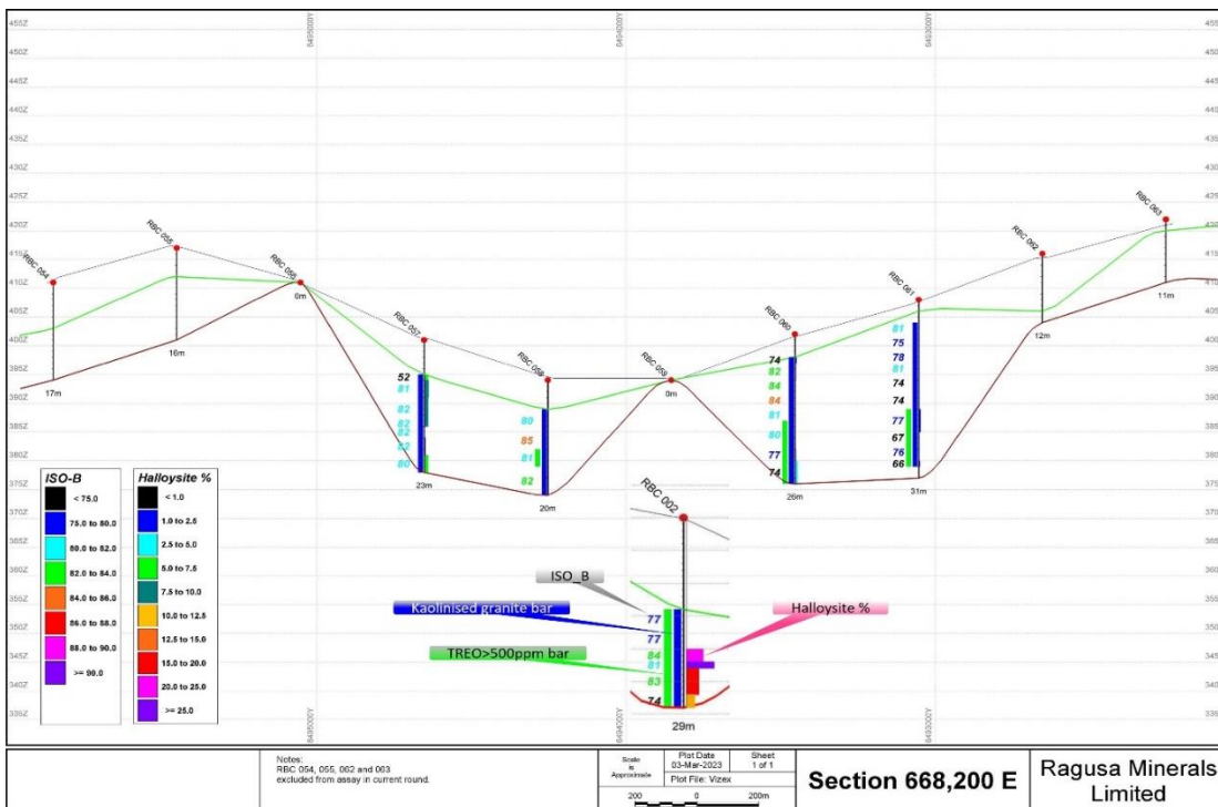
Figure 2. Section 668,200 East
