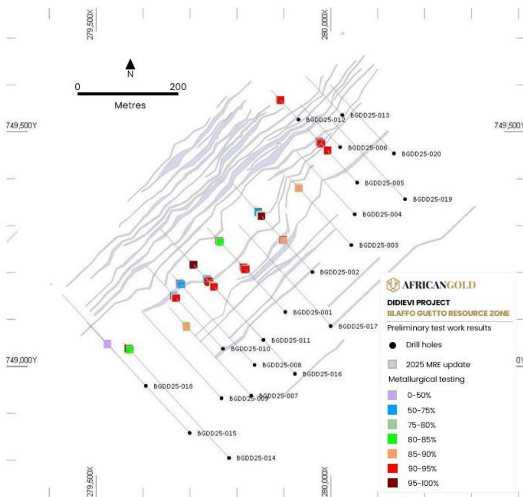
Figure 2: Plan view of metallurgical testing results across the Blaffo Guetto Resource
