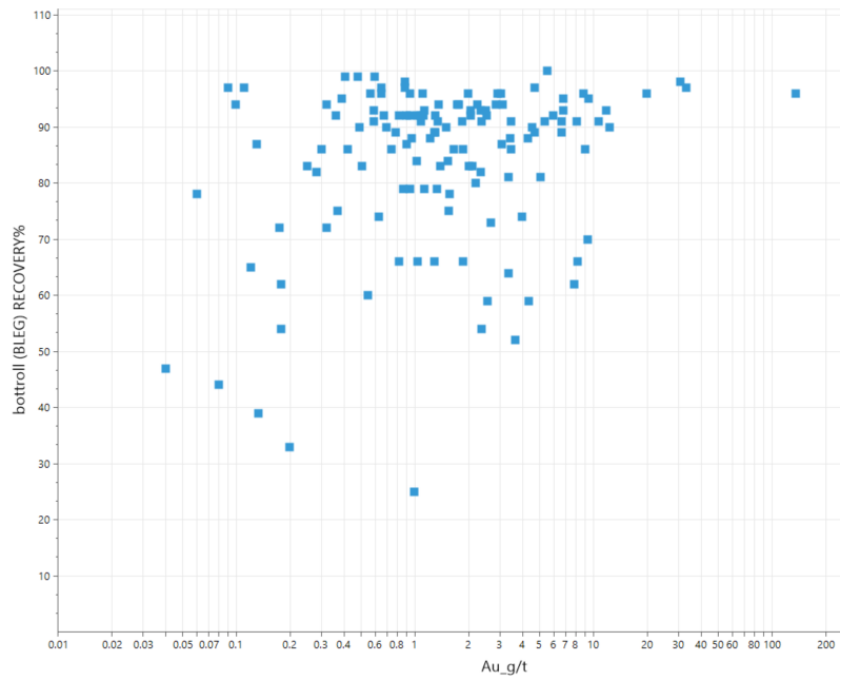
Fig 1.9-4: Recovery% vs gold grade (Au g/t) of the tested samples
