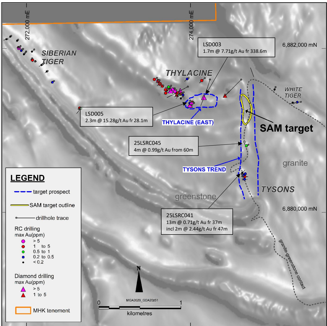
Figure 2. Aeromagnetic image (TMI) showing all MHK drilling at Leinster South, maximum gold values, SAM conductor and target prospects
